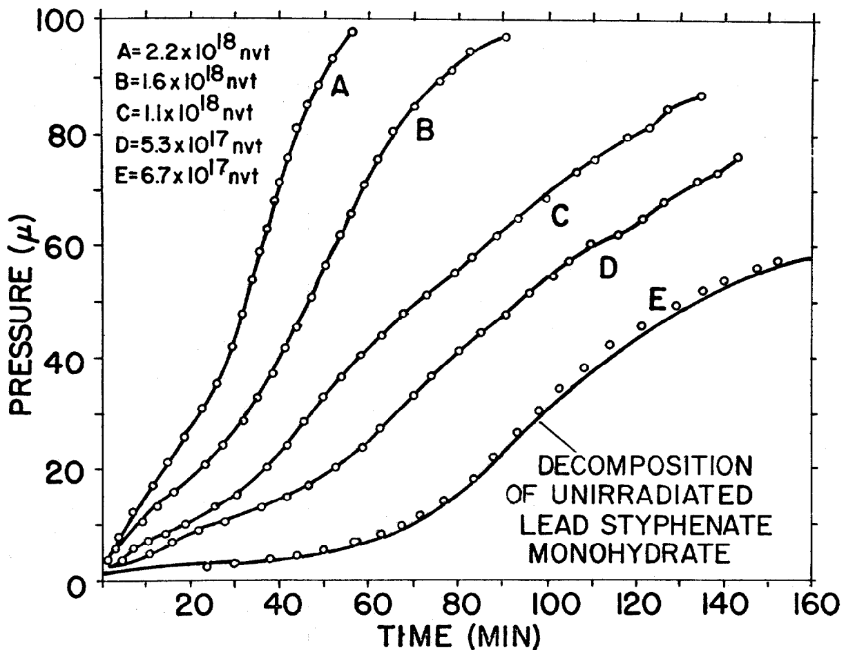
Fig 3 The Thermal Decomposition Curves of Reactor-Irradiated Pb Styphnate Monohydrate ( 222.5^\circ ) (Ref 61)
